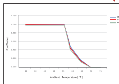
溫度降額特性 Temperature derating characteristics
